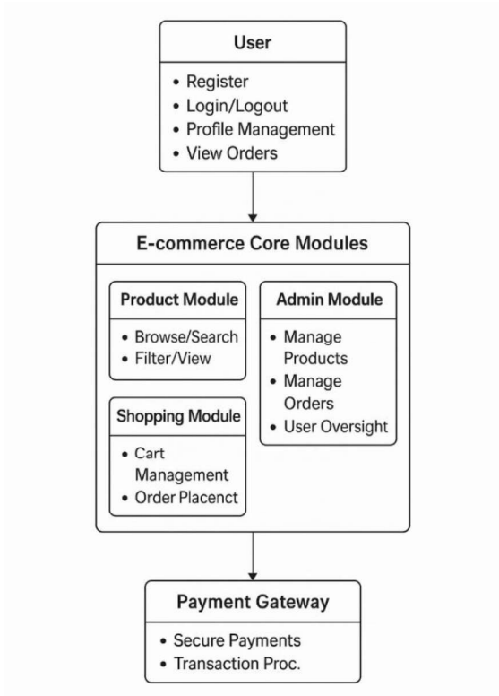
Figure 2: Relationships within the E-commerce System
